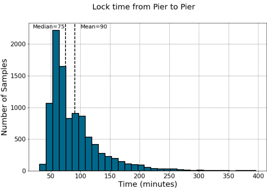
Figure 3: Transit times between approach piers (Zones 4 and 6) through the Soo Locks.
